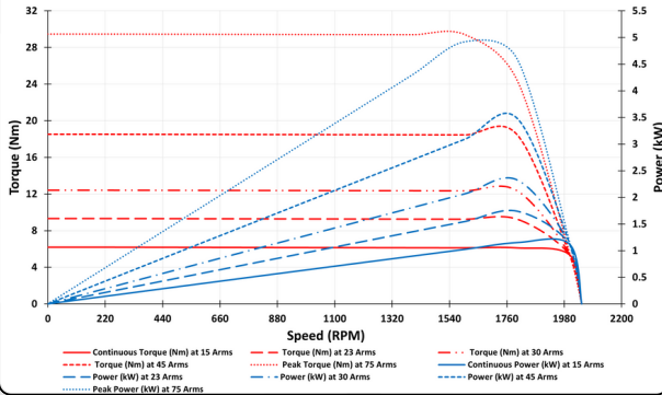
Performance curve 145-FZS72-015
