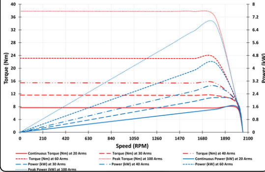
Performance curve 145-HZS72-020
