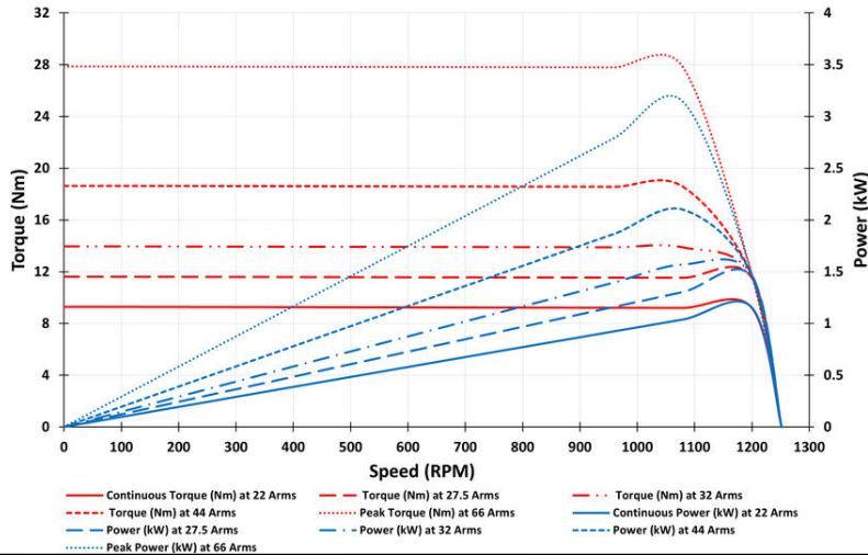
Performance curve 145-AZZS48-022
