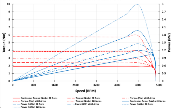
Performance curve 145-BZS24-040
