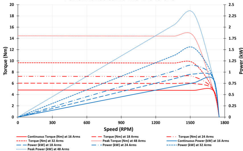
Performance curve 145-EZS48-016
