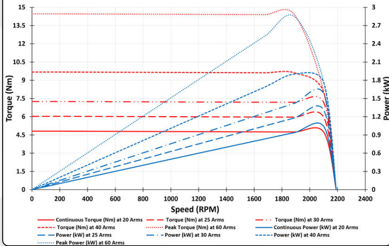
Performance curve 145-EZS48-020
