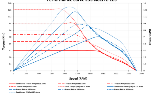
Performance curve 255-ACZI72-125
