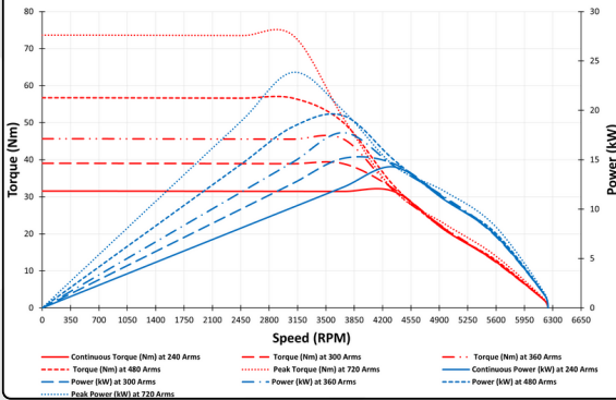
Performance curve 255-AZZI72-240
