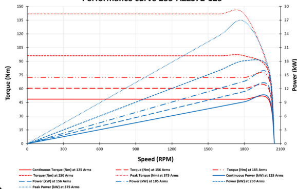
Performance curve 255-AZZS72-125
