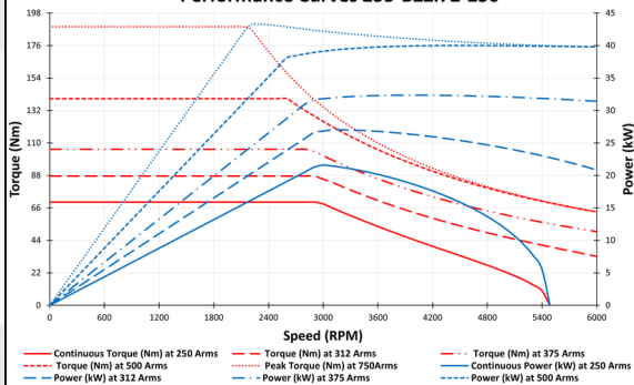
Performance Curves 255-BZZI72-250
