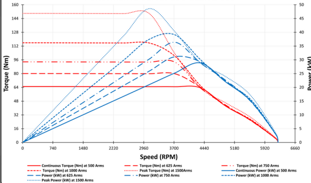
Performance Curves 255-BZZI72-500
