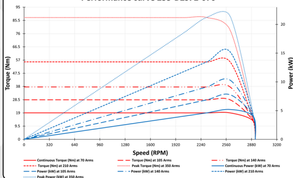
Performance curve 255-DZS72-070
