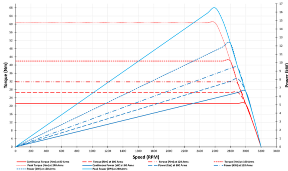
Performance Curves 255-DZS72-080
