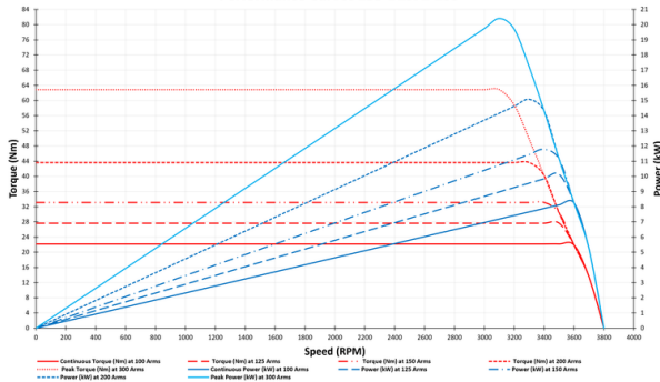
Performance Curves 255-DZS72-100
