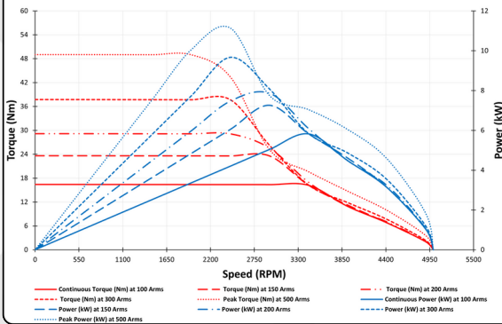
Performance curve 255-EZ172-100
