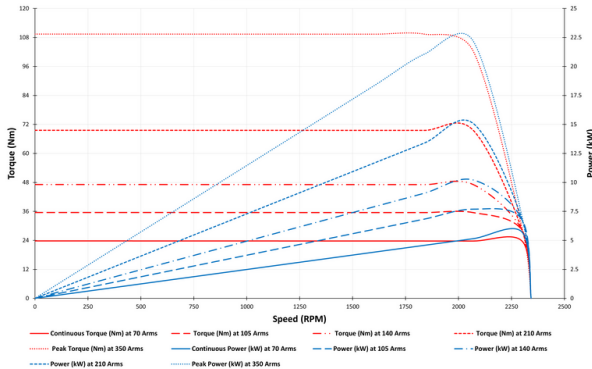
Performance Curves 255-EZS72-070
