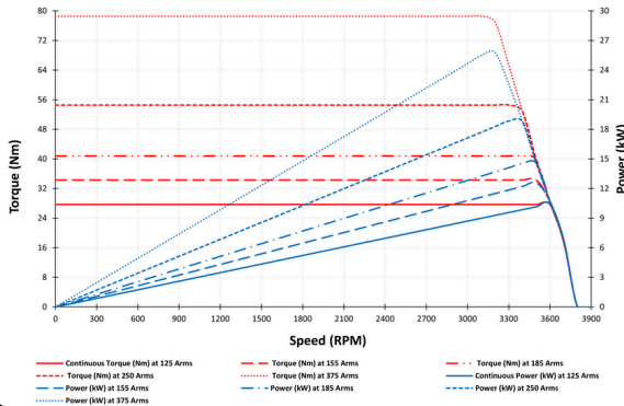
Performance curve 255-EZS72-125
