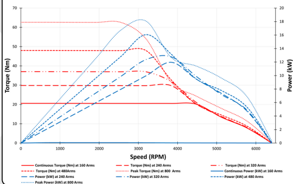
Performance curve 255-FEI72-160
