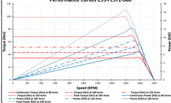
Performance Curves 255-FES72-080
