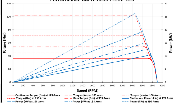
Performance Curves 255-FES72-125
