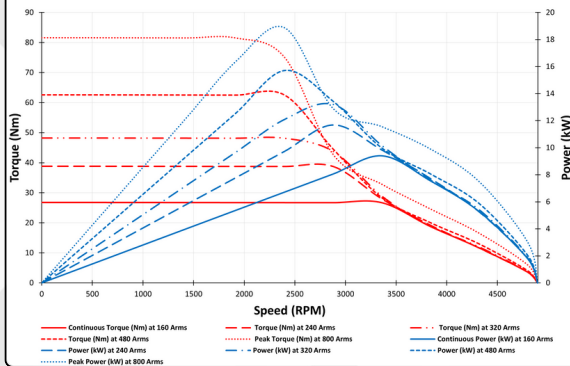
Performance curve 255-HEI72-160
