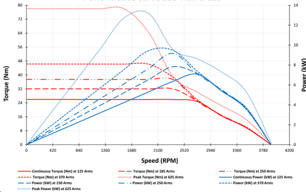
Performance curve 255-HZ172-125
