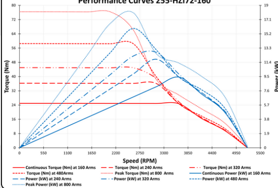
Performance Curves 255-HZ172-160
