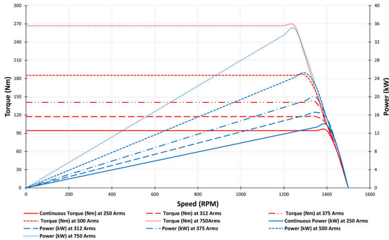
Performance Curves 255-AGZS48-250
