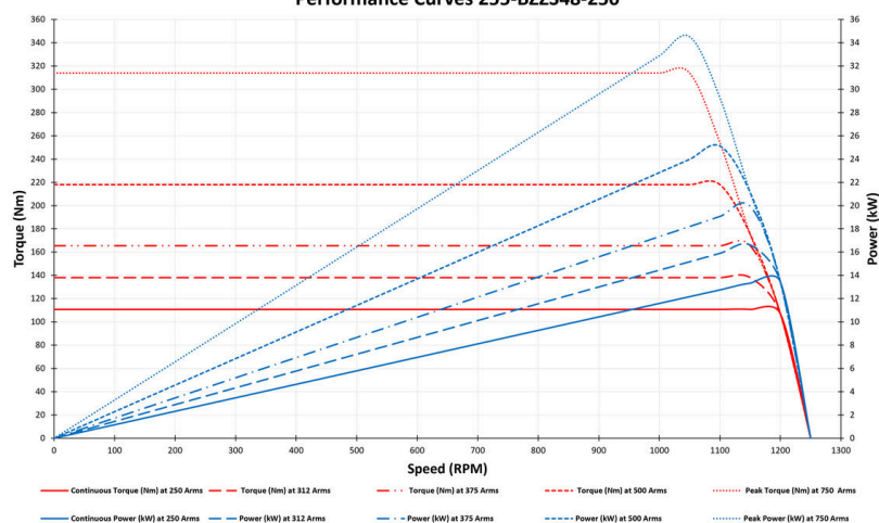
Performance Curves 255-BZZS48-250
