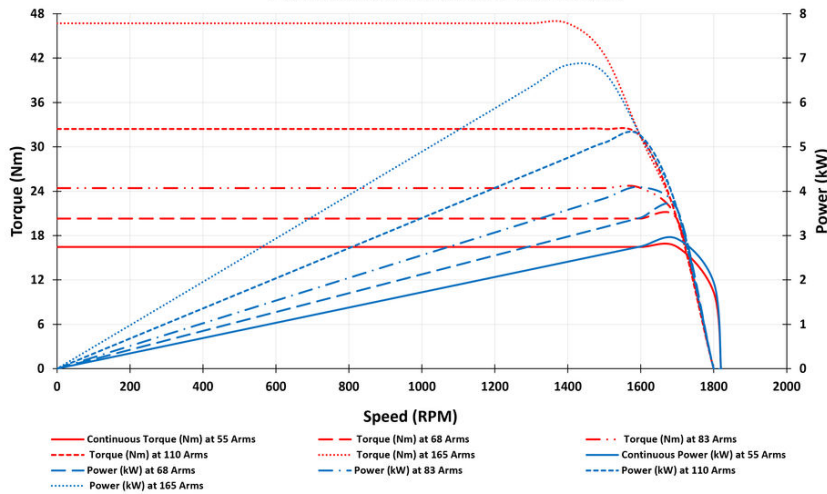
Performance curve 255-CZS48-055
