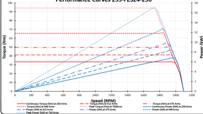
Performance Curves 255-FZS24-250
