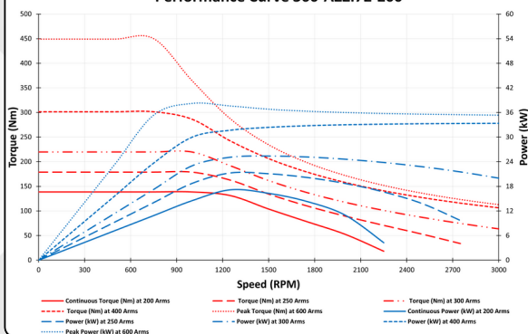
Performance Curve 360-AZZI72-200
