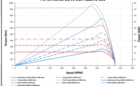
Performance curve 360-AZZS72-200
