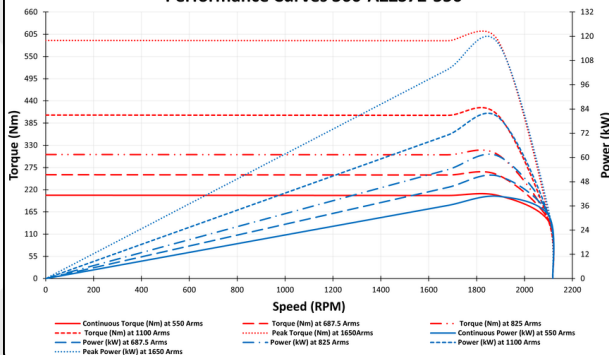
Performance Curves 360-AZZS72-550
